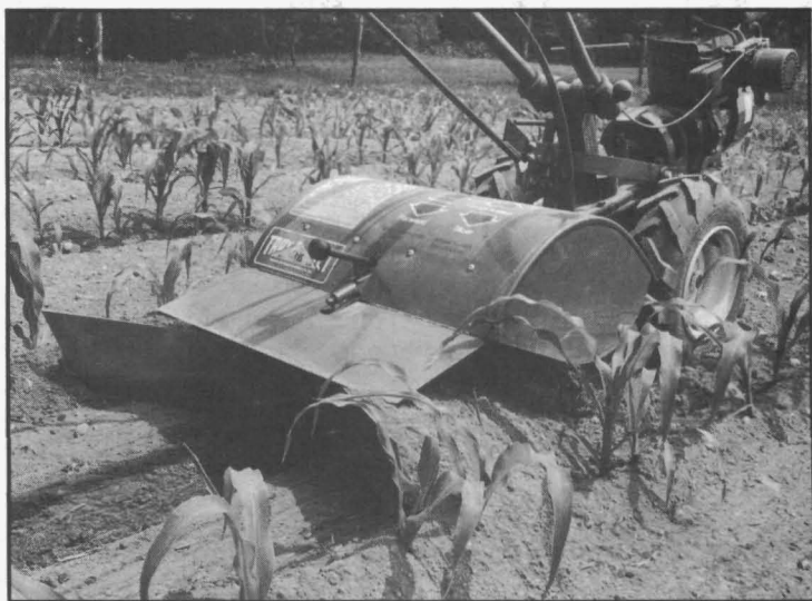
Hiller/Furrower weeds as it hills.
