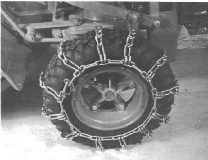
If you have the older 7-inch, cast-iron, spoked wheels as shown above, use Part No. 9139 Chains.
