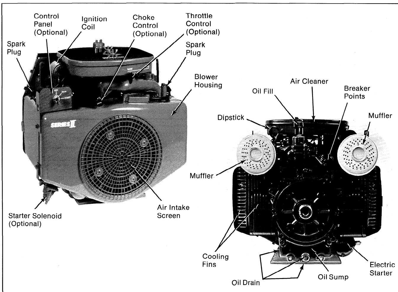
Figure 1. Typical KT Engine.
