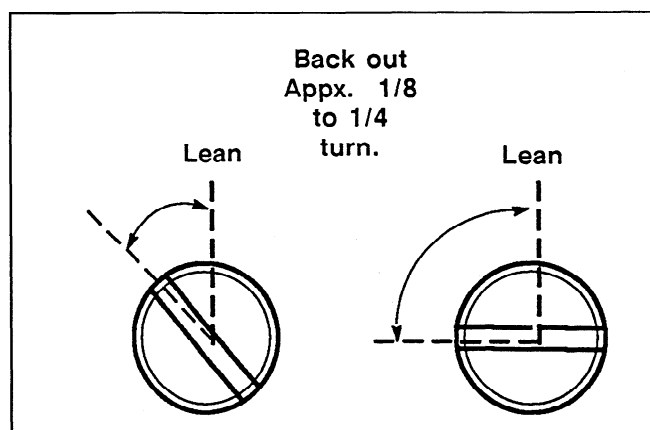
Figure 12. Optimum Low Idle Fuel Setting.
