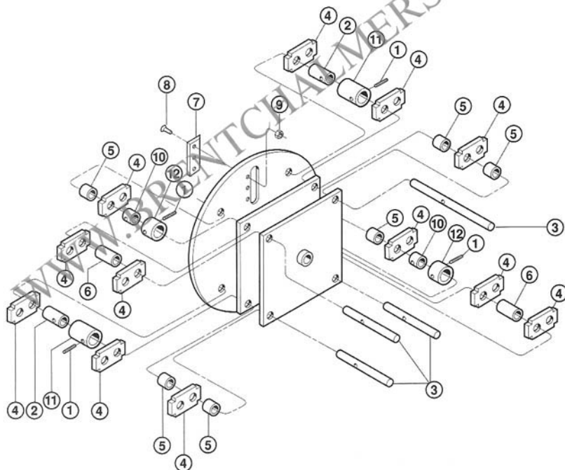
Cylinder Assembly — 5HP & 8HP Non-I/C Models Only
